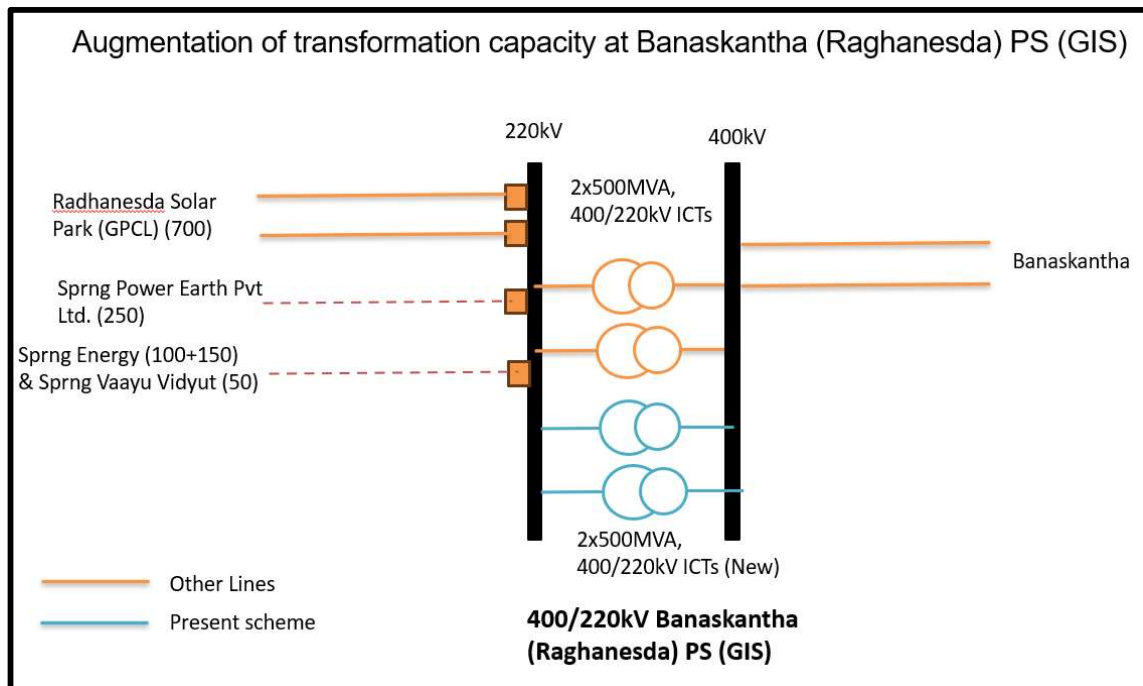
Fig-1: Augmentation of transformation capacity at Banaskantha (Raghnesda) PS (GIS)
