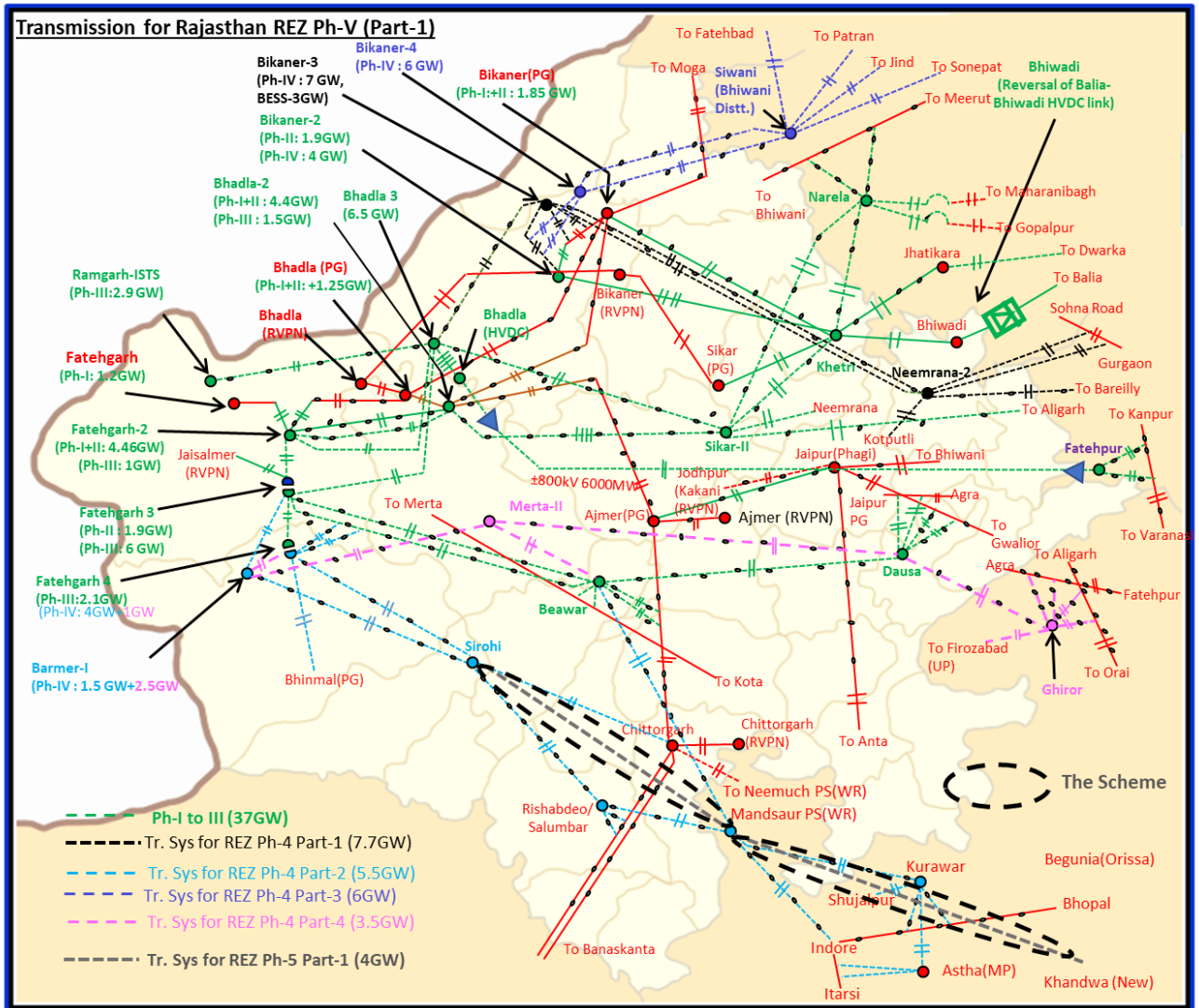
Fig-1: Transmission system for evacuation of power from Rajasthan REZ Ph-V (Part-1: 4 GW) [Sirohi/Nagaur] Complex
