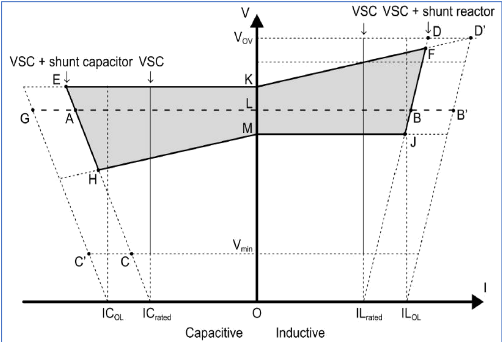
Figure-3: VI Curve of the STATCOM Station
