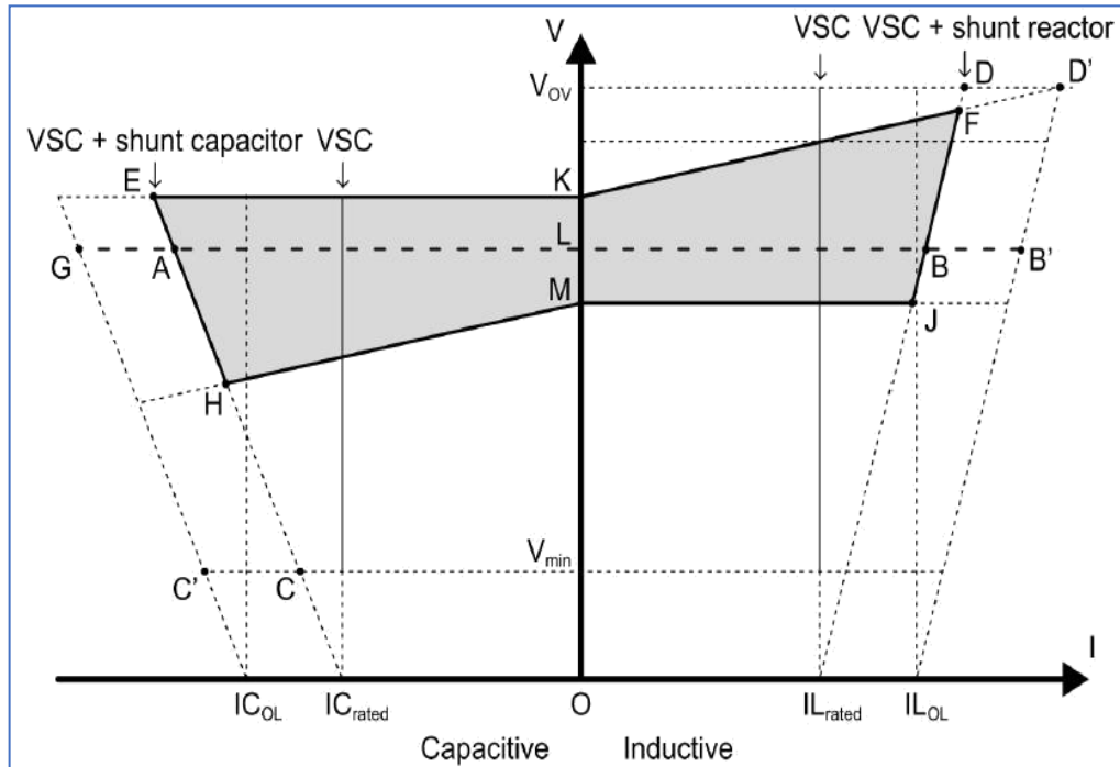
Figure-3: VI Curve of the STATCOM Station
