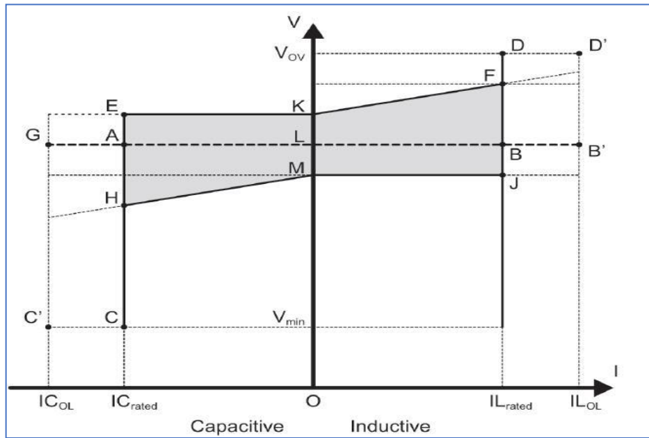
Figure-2: VI Curve of the VSC Portion
