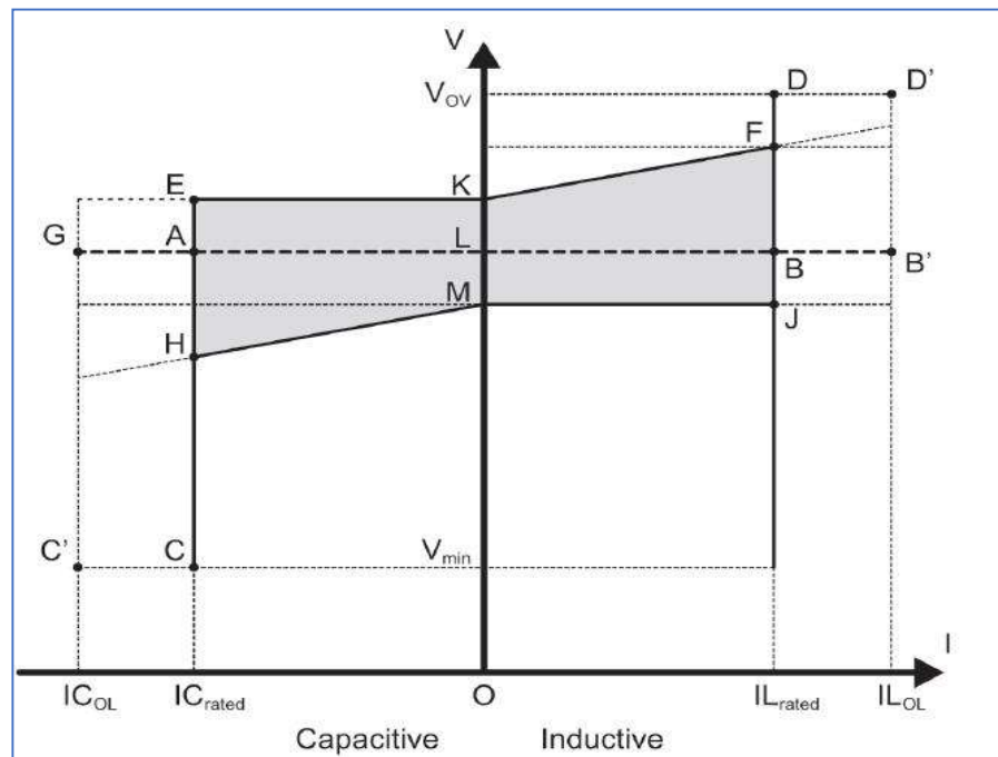
Figure-2: VI Curve of the VSC Portion
