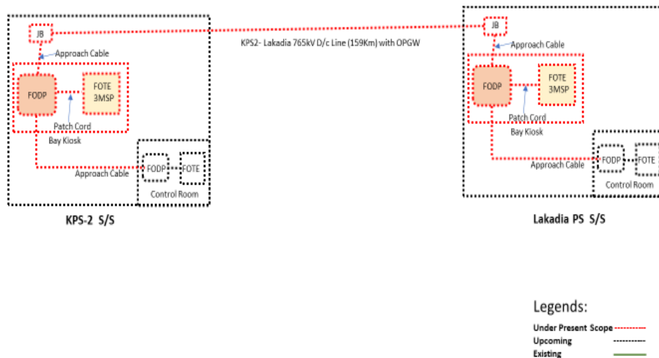
Proposed Communication for Transmission scheme for evacuation of 4.5 GW RE injection at Khavda PS under Phase-II - Part A
